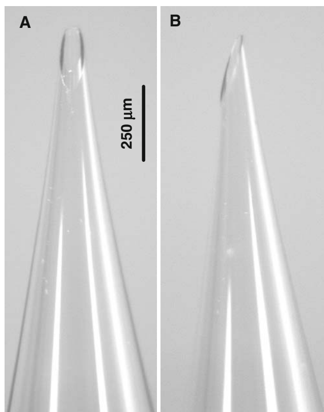
Fig. 1. Representative hollow microneedle: a front view and b side view. The microneedle shown has an approximately elliptical tip opening with a long axis of ~100 μm and a short axis of ~40 μm with a bevel tip angle of 25°.
